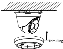
Figure 2-8 Install the Trim Ring
