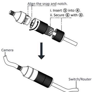
Figure 2-44 Waterproof Accessory Installation
